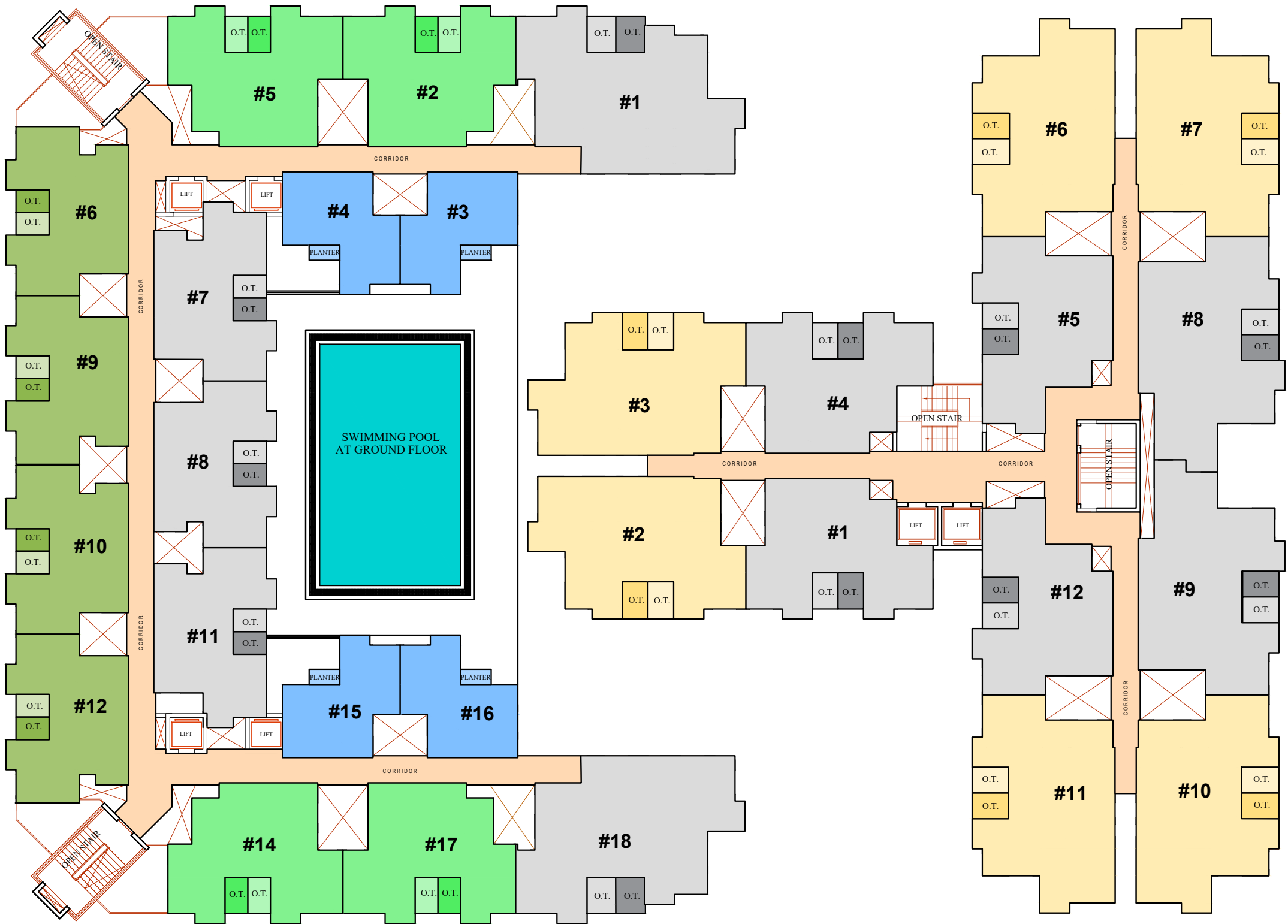
TYPICAL FLOOR PAN ( 1ST. TO 12TH. FLOOR PLAN )
